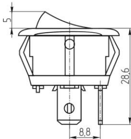
Mounting
