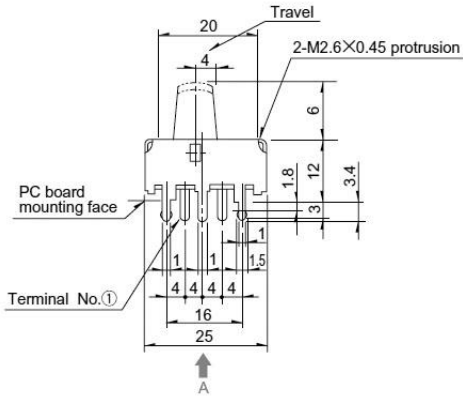
Outline Drawing
