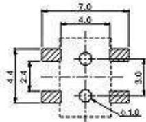
Mounting
